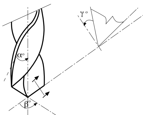
Regular Drill Bit
