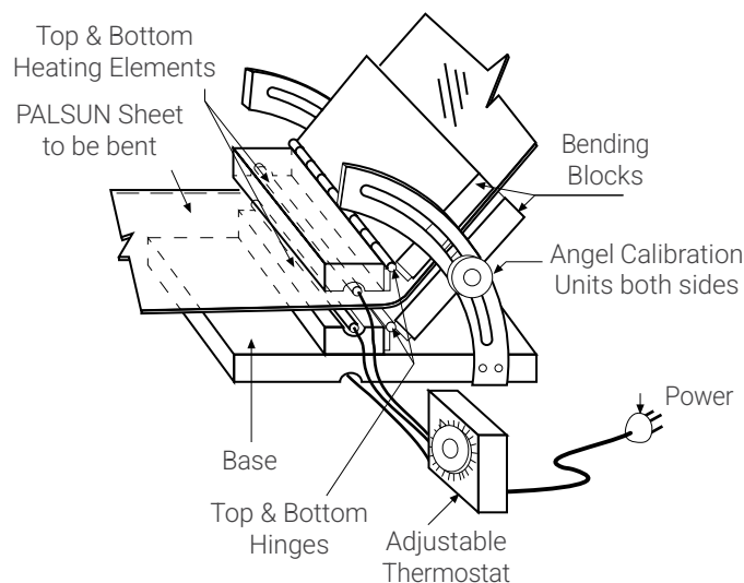
Heat bending device
